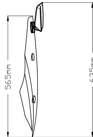
TOURING SCREEN WITH VISOR AT UPPER POSITION
