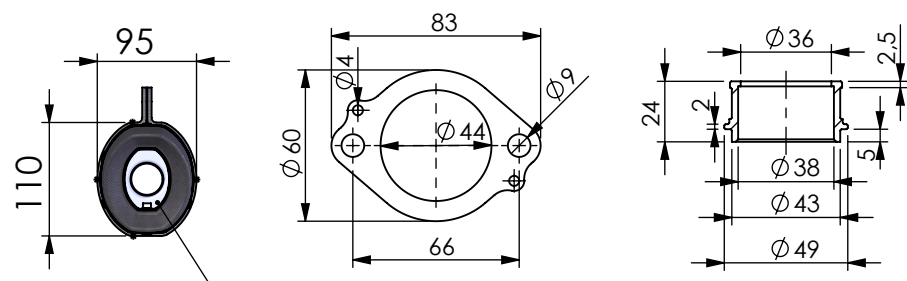
s.s. Flange "108B" cod.204835 sp.5mm
