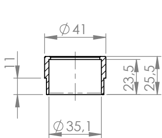
Bushing Cod.206060
